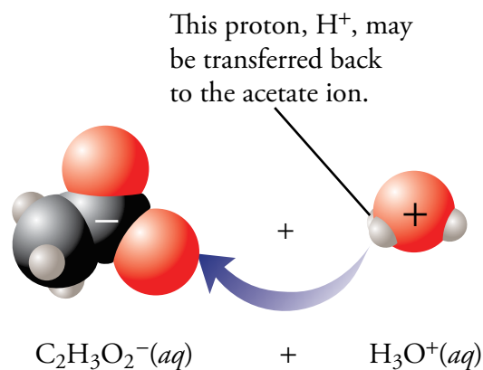
Figure 6.5 Reversible Reaction of Acetic Acid and Water
